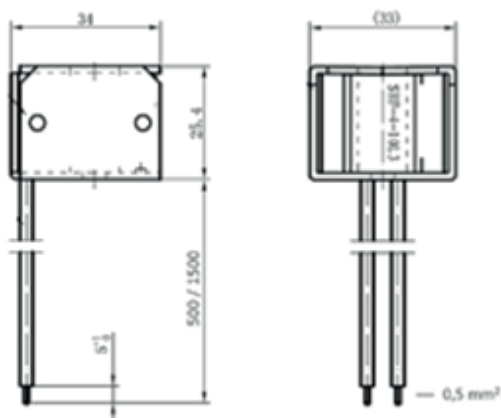
Bobinas com cabos (SQ-A25 Series)
